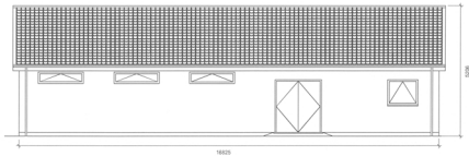
west elevation
